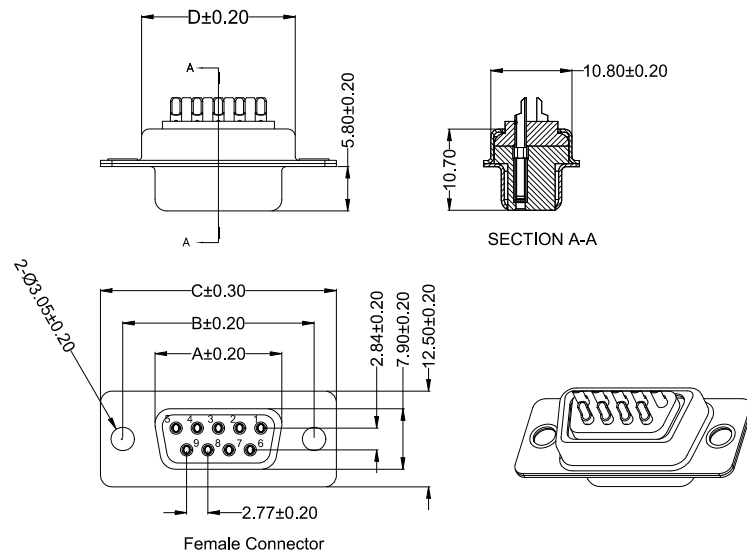
Female connector
