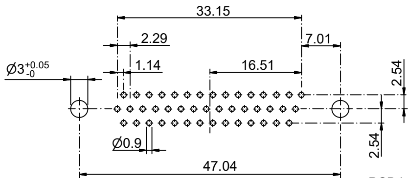
PCB Layout tolerances +/-0.1
