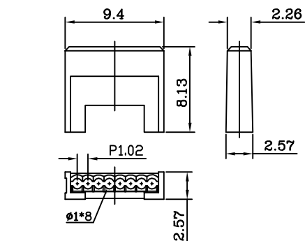
PLUG 8P8C Insert
