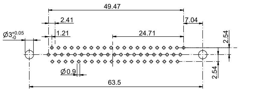
PCB Layout tolerances ±0.1
