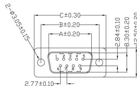
Male Connector
