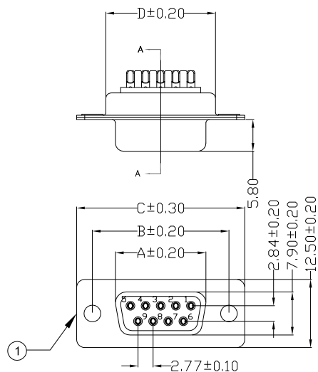
Famale Connector
