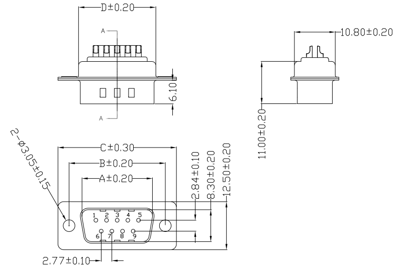
Male Connector
