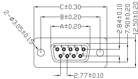
Female Connector
