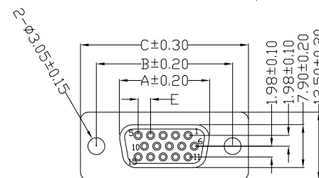
Female Connector
