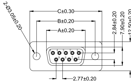
Female Connector
