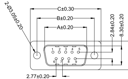
Male Connector
